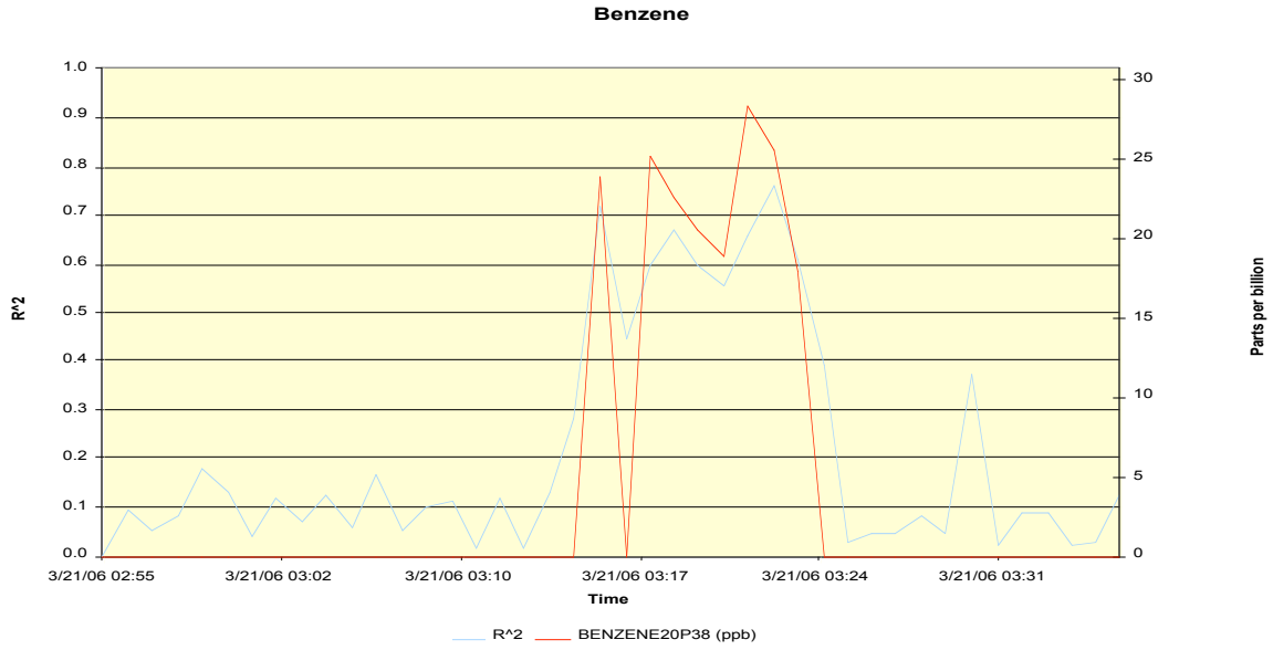
Figure 2 - Plot of Benzene Concentration in parts per billion versus time
